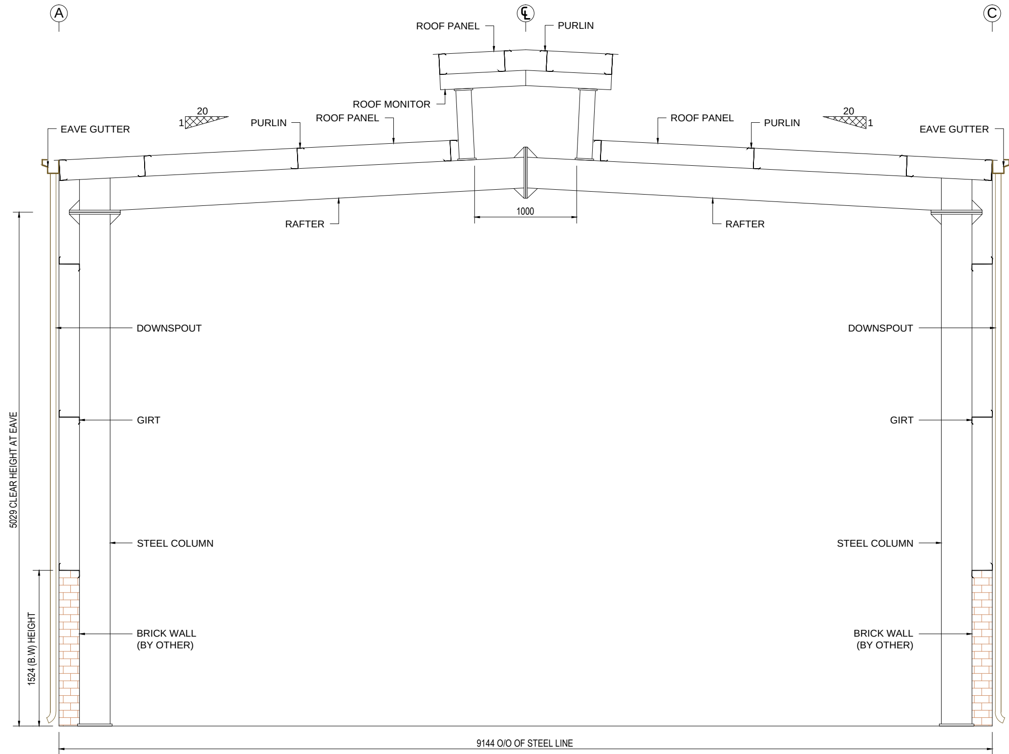
CROSS SECTION
